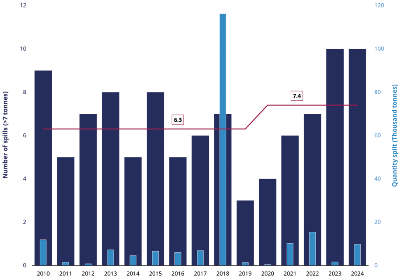
FIGURE 15: NUMBER OF TANKER SPILLS AND QUANTITIES OF OIL SPILT (>7 TONNES) FROM 2010-2024
