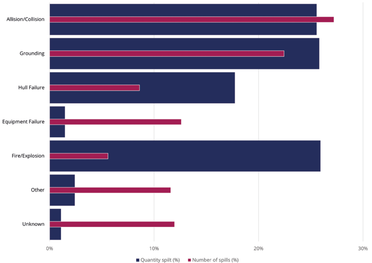
FIGURE 11: NUMBER OF TANKER SPILLS AND QUANTITY SPILT PER CAUSE, 1970-2024
