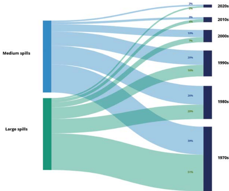
FIGURE 5: MEDIUM (7-700 TONNES) AND LARGE (>700 TONNES) TANKER SPILLS AS A PERCENTAGE OF THOSE RECORDED PER DECADE, 1970-2024
