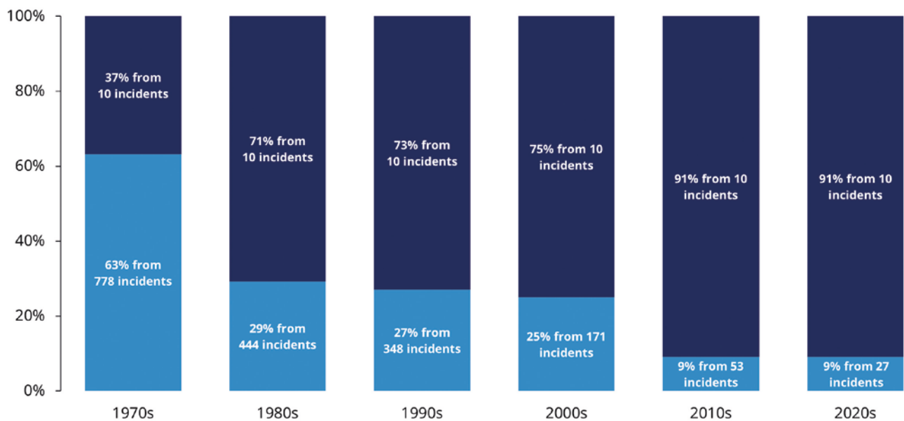
FIGURE 7: TANKER SPILLS 7 TONNES AND OVER PER DECADE SHOWING THE INFLUENCE OF A RELATIVELY SMALL NUMBER OF COMPARATIVELY LARGE SPILLS ON THE OVERALL FIGURE
