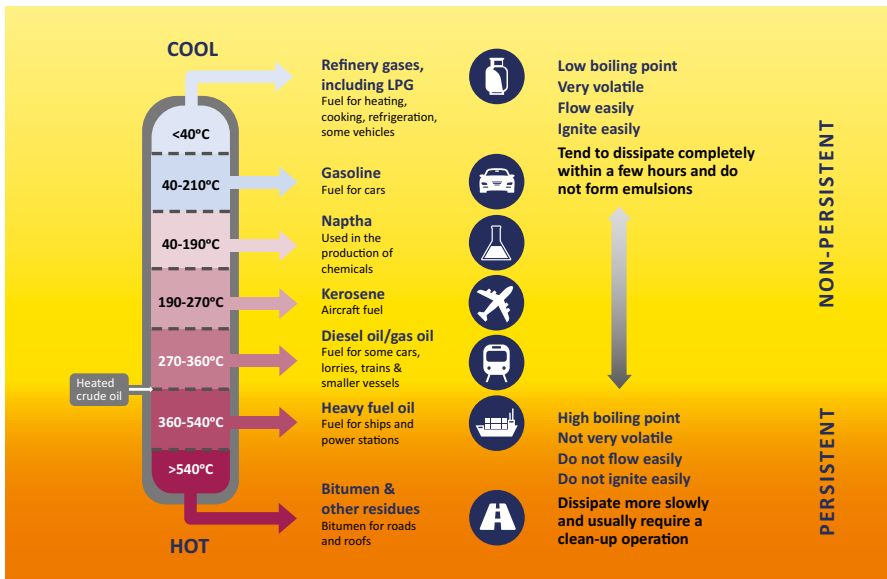
CRUDE OIL AND ITS DISTILLATION FRACTIONS
